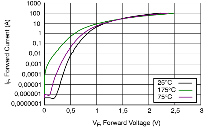
Figure 16. Forward Characteristics
