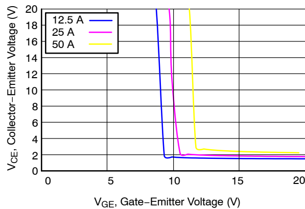
Figure 5. Saturation Voltage vs. V_{GS} (25°C)
